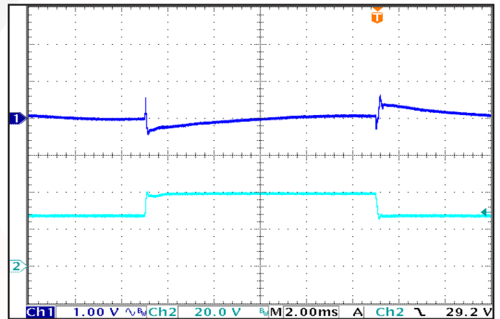
Figure 12: Output Voltage Response to Step-Change in Input Voltage , ( dV/dt = 250 V/ms). Load capacitance: 1 μF ceramic and 100 μF electrolytic capacitors. Ch 1: \Delta V_{out} (1 V/div); Ch 2: V_{in} (20 V/div); Timescale: 2.00ms/div.
