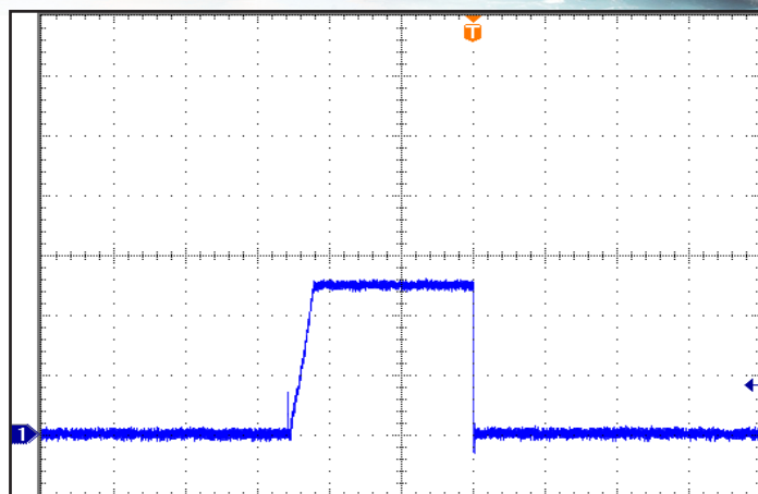
Figure 14: Output Short Load Current , (20 A/div) as a function of time (20 ms/div) when the converter attempts to turn on into a 1 mΩ short circuit. Timescale: 20.0ms/div.
