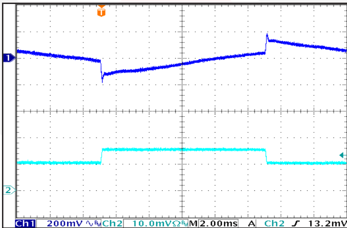
Figure 11: Output Voltage Response to Step-Change in Load Current , (50-75-50% of I_{out(max)} ; di/dt = 0.1 A/μs). Load capacitance: 1 μF ceramic and 100 μF electrolytic capacitors. Ch 1: \Delta V_{out} (200 mV/div); Ch 2: I_{out} (20 A/div); Timescale: 2.00ms/div.
