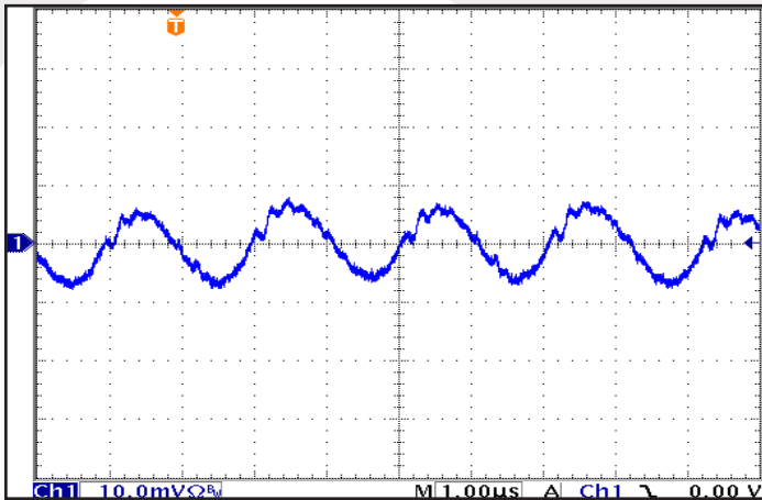
Figure 9: Input Terminal Current Ripple , i_C , at full rated output current and nominal input voltage with SynQor MCOTS filter module (2 A/div). Bandwidth: 20 MHz. Timescale: 1.00μs/div. See Figure 13.
