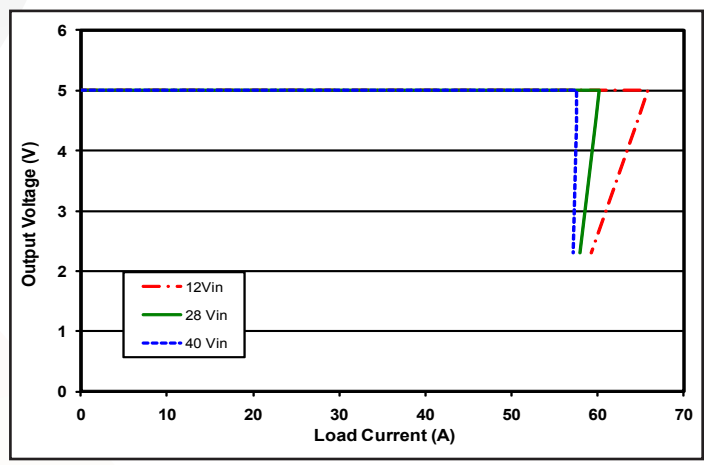
Figure 6: Output I-V Characteristics , (output voltage vs. load current) showing typical current limit curves. See Current Limit section in the Application Notes.
