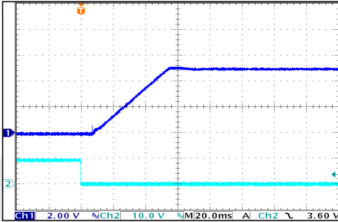
Figure 7: Typical Startup Waveform , input voltage pre-applied. Ch 1: V_{out} (2 V/div); Ch 2: ON/OFF Pin (10 V/div); Timescale: 20.0ms/div.
