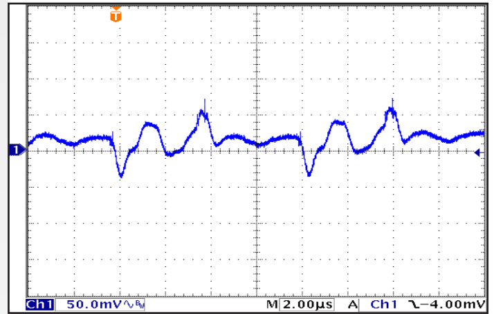
Figure 10: Output Voltage Ripple , V_{out} , at nominal input voltage and rated load current (50 mV/div). Load capacitance: 1 μF ceramic and 100 μF electrolytic capacitors. Timescale: 2.00μs/div. Bandwidth: 20 MHz. See Figure 13.
