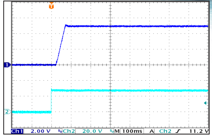
Figure 8: Turn-On Transient , at full resistive load and zero output capacitance, initiated by V_{in} . Ch 1: V_{out} (2 V/div); Ch 2: V_{in} (20 V/div); Timescale: 100ms/div.
